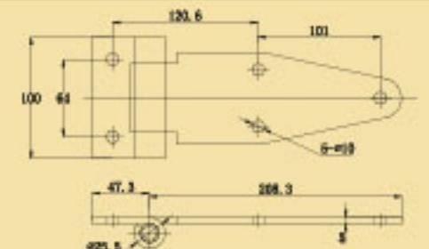
Strap Hinge Steel Zinc Plated
