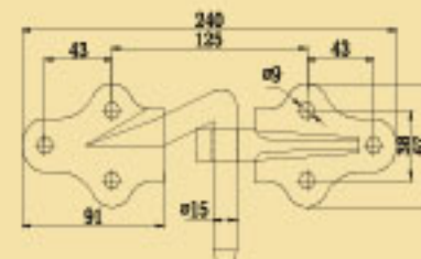
Stake Body Hardware Malleable Iron Zinc Plated
