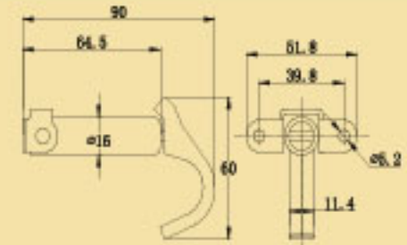
Hood Catch Spring Loaded Steel Black Enamel
