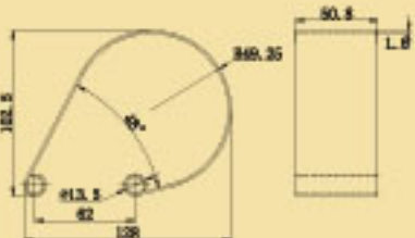
Spring Door Stoppers Plain Steel
