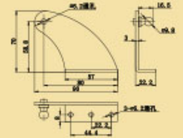
Ball End Fittings And Stud S/S Steel
