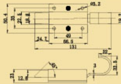
Finger end Bolts Steel Zinc Plated
