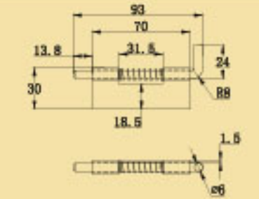
Spring-Loaded Bolts Steel Zinc Plated
