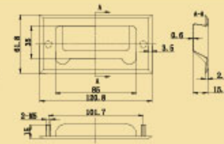
Recessed Handle
