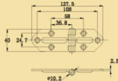
Stamped Stainless Steel 304. 316 Hinge
