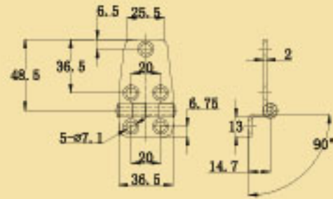
Stamped Stainless Steel 304. 316 Hinge
