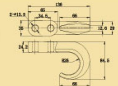
Tow Hook Forg Steel Black Enamel
