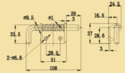
Latch Hinge With Spring Steel Zinc Plated S/S
