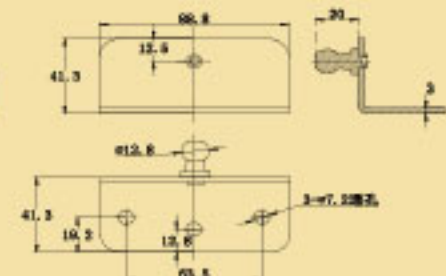
Ball End Fittings And Studs Steel Zinc Plated S/S 304
