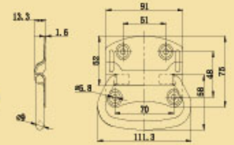
Chest Handles Zinc Plated In Steel 90 Degree Stop
