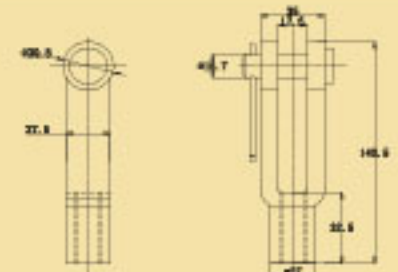
Yoke Rod Ends And Pins Forged Steel Zinc Plated
