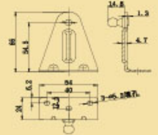
Ball End Fittings And Studs Steel Zinc Plated S/S 304
