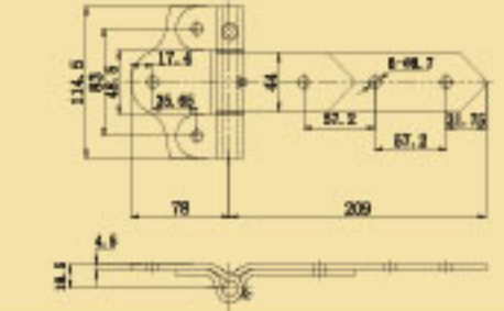
Strap Hinge Zinc Plated Steel
