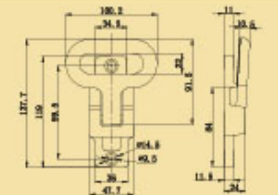
Folding Step Casting Steel Zinc Plated
