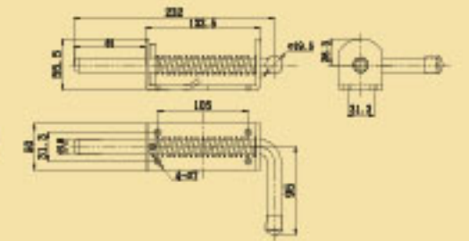
Spring Bolts Steel Zinc Plated
