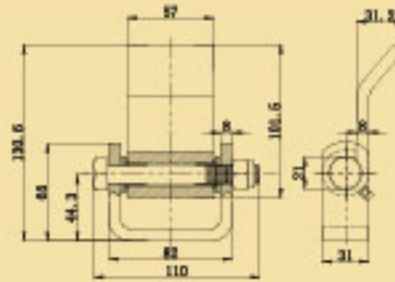
Strap Hinge Plain Steel
