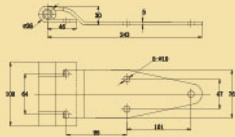
Strap Hinge Steel Zinc Plated
