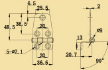
Stamped Stainless Steel 304. 316 Hinge
