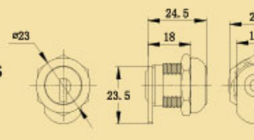
Cylinders Locks
