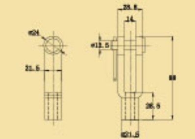
Yoke Rod Ends And Pins Forged Steel Zinc Plated
