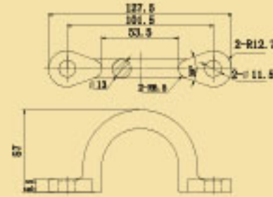
Aluminum Handle
