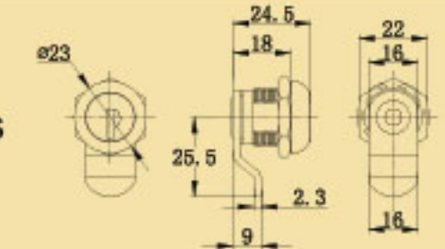
Cylinders Locks
