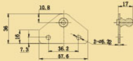
Ball End Fittings And Stud Steel Zinc Plated S/S 304
