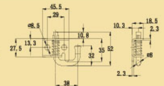
Spring Bolts Steel Zinc Plated
