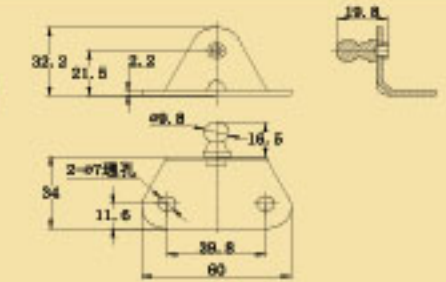
Ball End Fittings And Studs Steel Zinc Plated S/S 304
