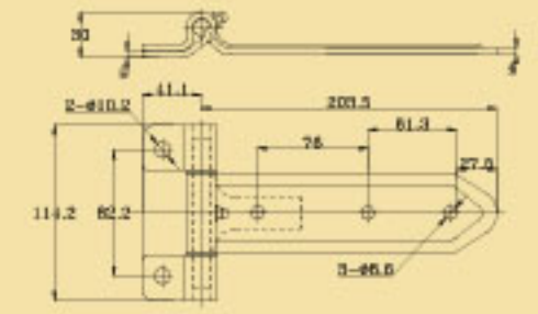
Strap Hinge Zinc Plated Steel
