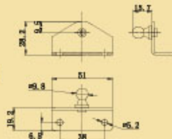
Ball End Fittings And Studs Zinc Plated Steel S/S 304
