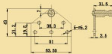
Ball End Fittings And Stud Steel Zinc Plated S/S 304
