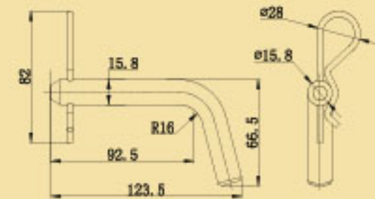
Hitch Pin Steel Zinc Plated
