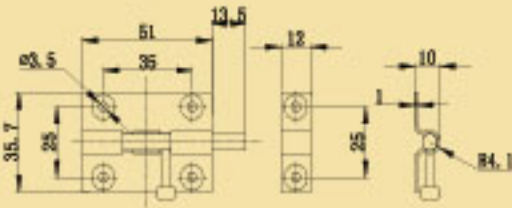
Barrel Bolts Steel Zinc Plated
