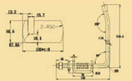
Spring Bolts Steel Zinc Plated
