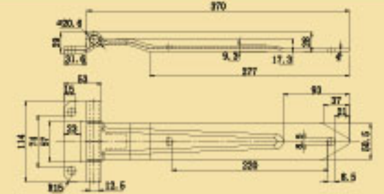
Strap Hinge Steel Zinc Plated
