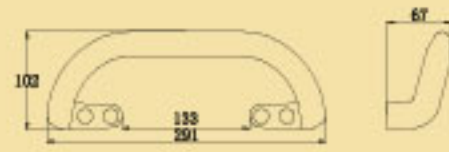
Grab Bars Poly Propylene Inside Steel
