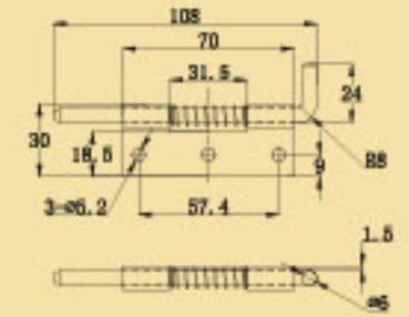
Spring-Loaded Bolts Steel Zinc Plated
