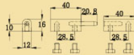
Block Hinge Lift-Off
